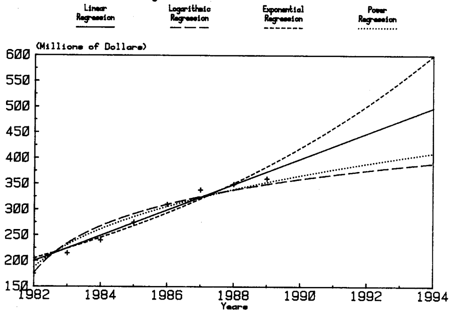
Curve Fit
