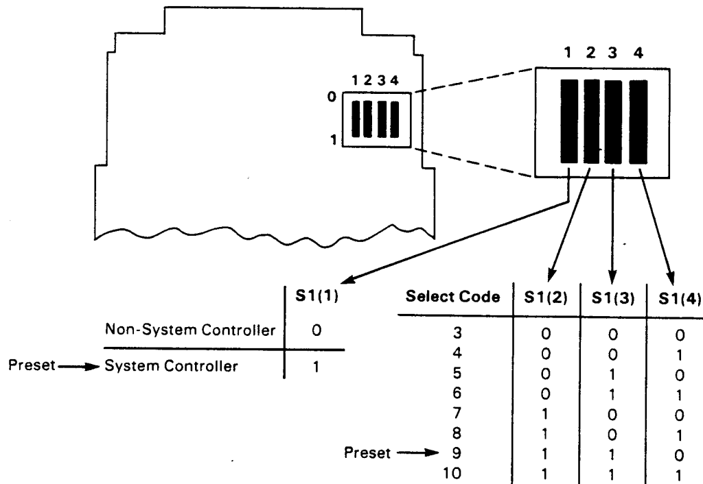
Figure 2-2. Switch Settings
