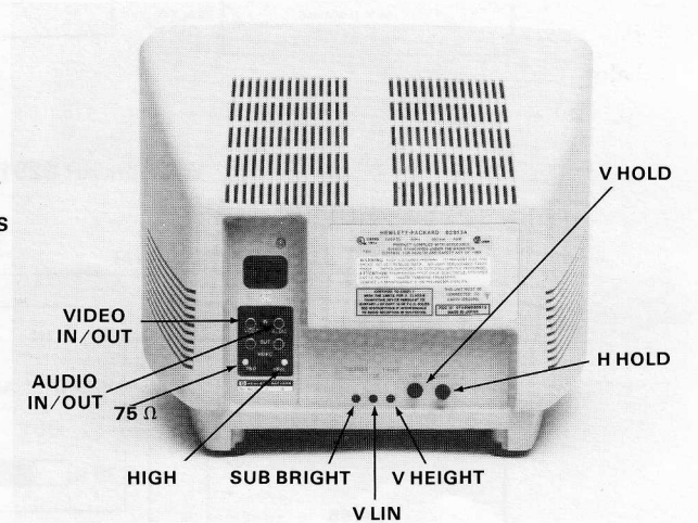
HP 82913A Video Monitor (12-inch)
