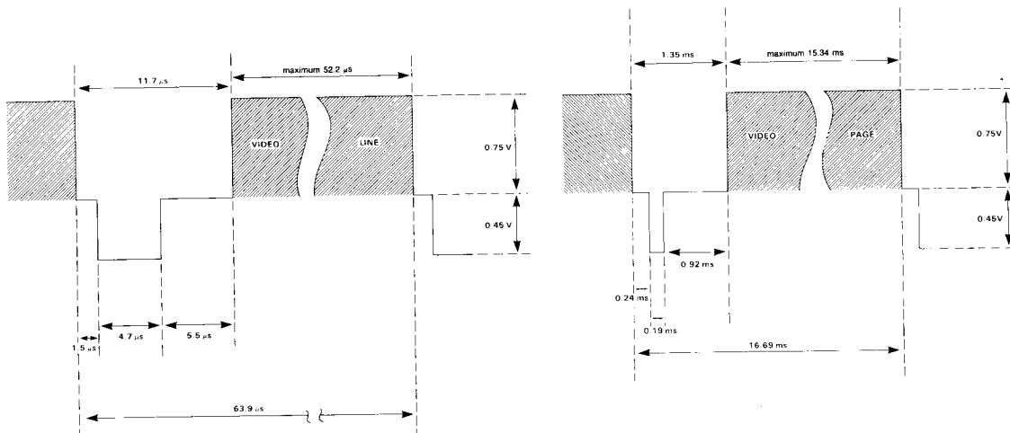
Vertical Composite Waveform
