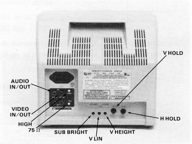
HP 82912A Video Monitor (9-inch)
