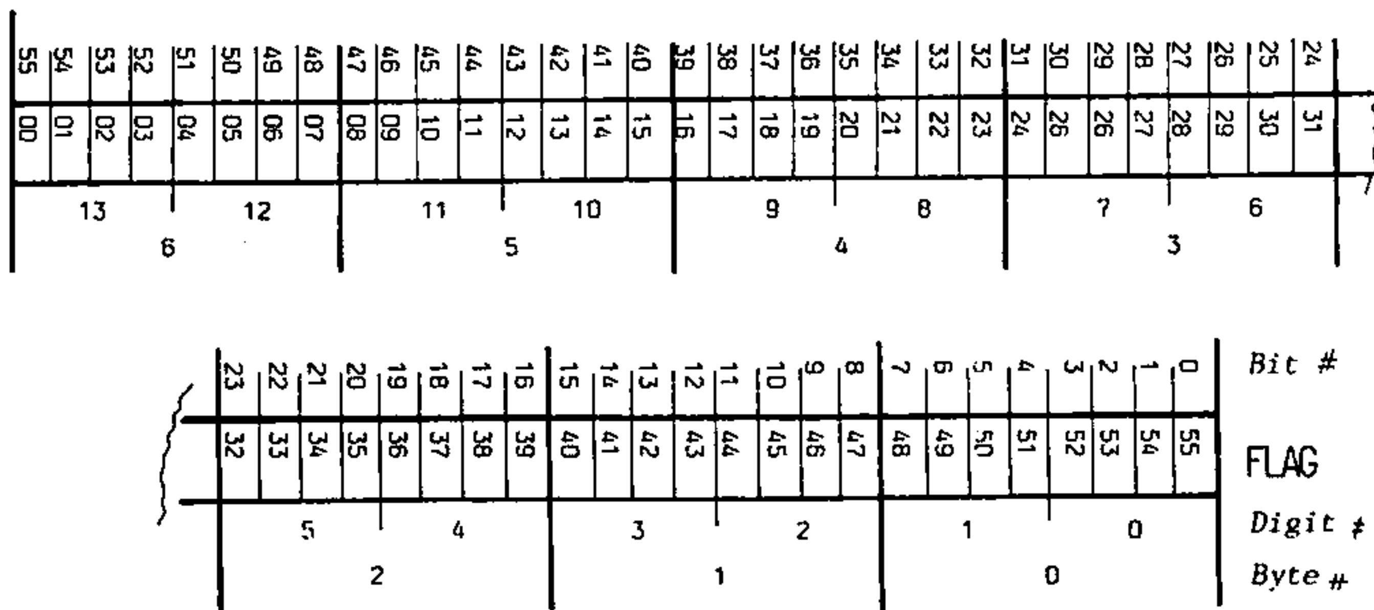
Figure 3.8.5 Flag Bit Locations in Register d
