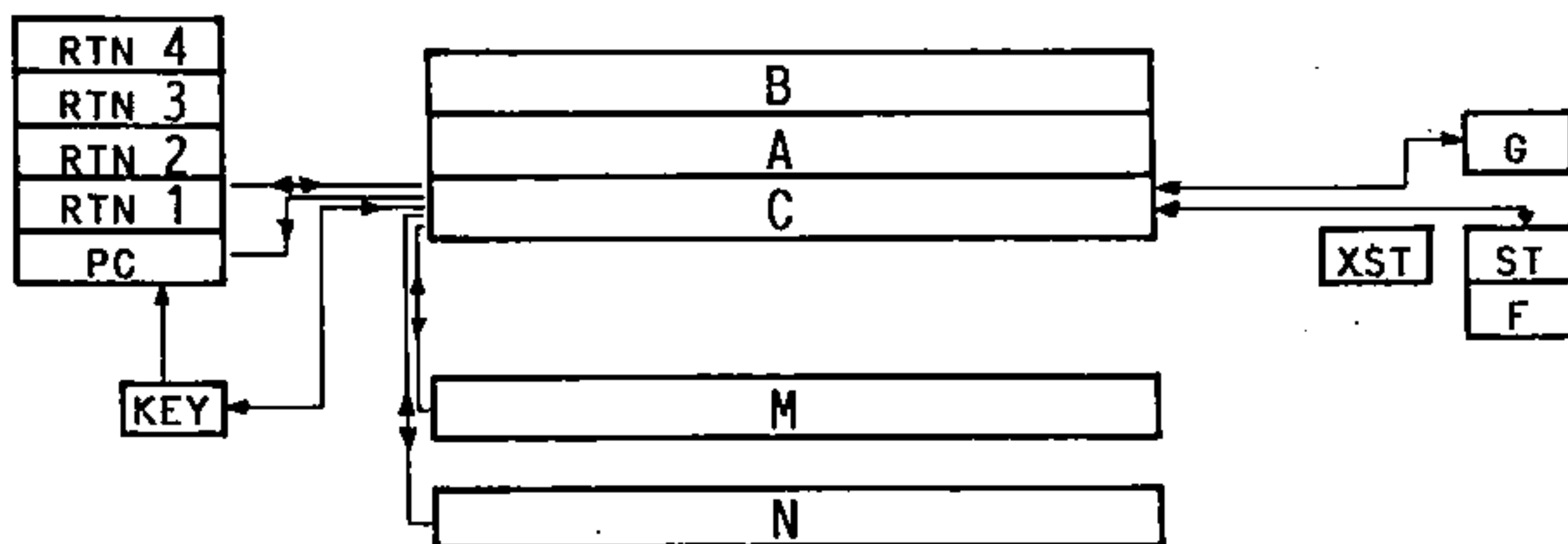
FIGURE 6.2.1. THE HP 41 CPU STRUCTURE
