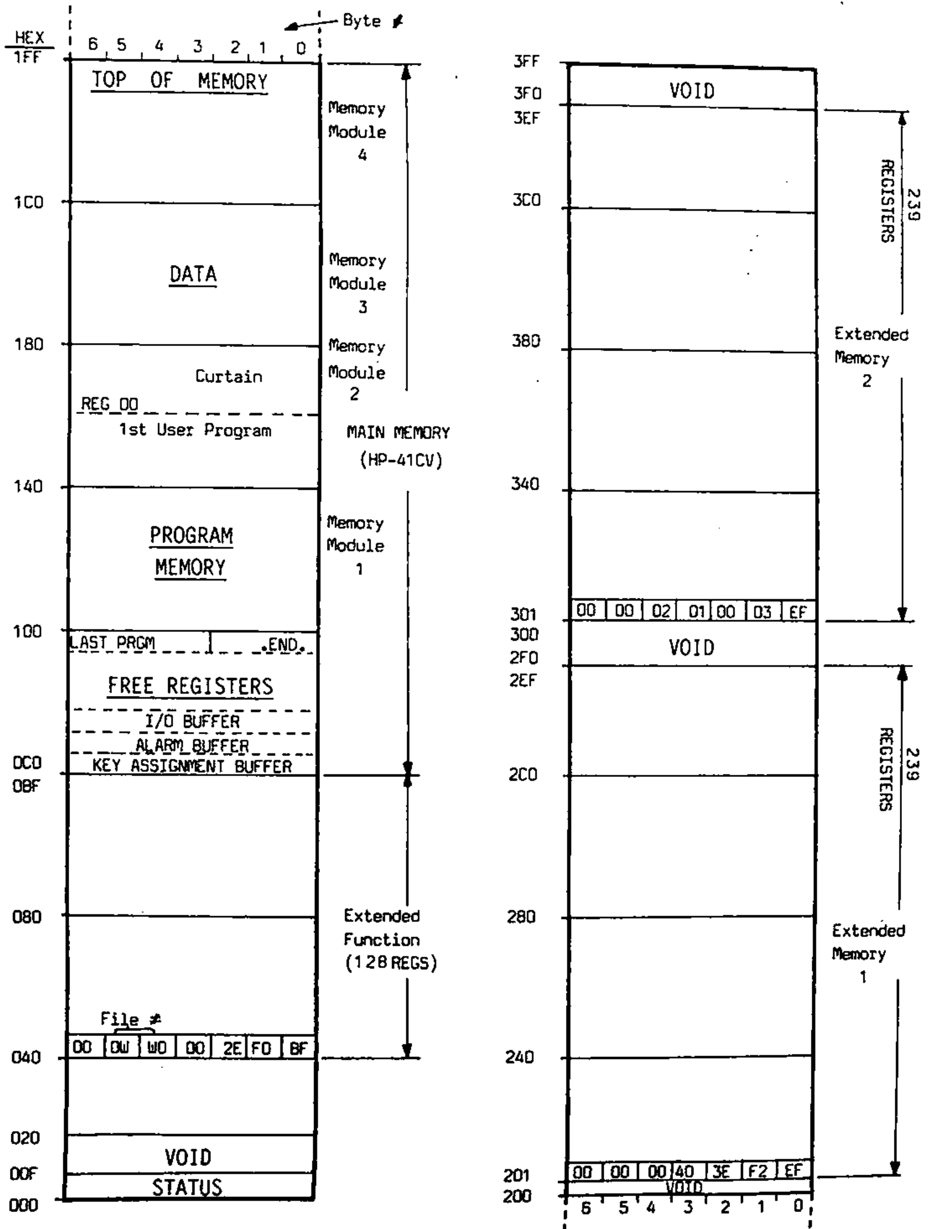
Figure 3.7.1 HP-41 Memory Configuration
