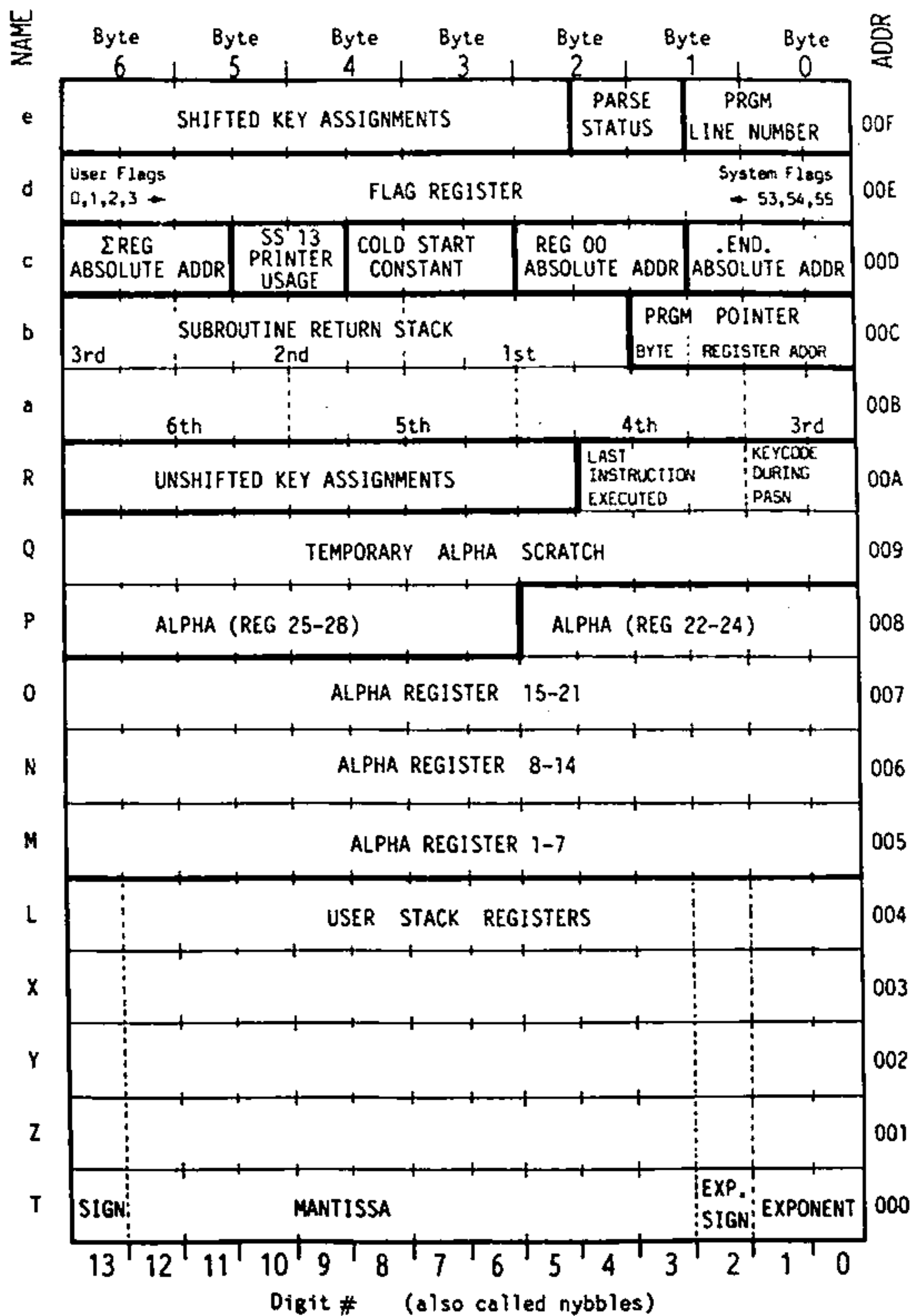
FIGURE 3.8.1 HP-41 STATUS REGISTERS
