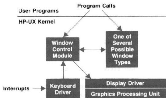
Fig. 3. Block diagram of intermodule connections for HP Windows in the Integral PC.
