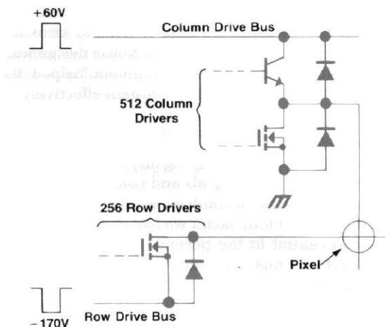
Fig. 5. Drive scheme used to excite the pixels on the Integral PC's electroluminescent display.
