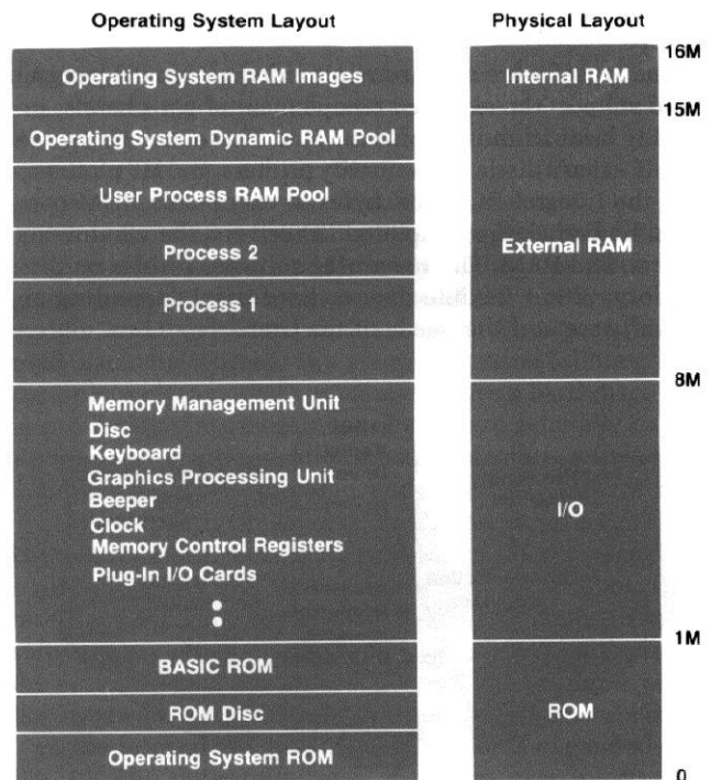
Fig. 3. Integral PC memory organization.
